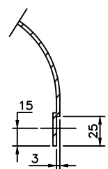
DETAIL X
